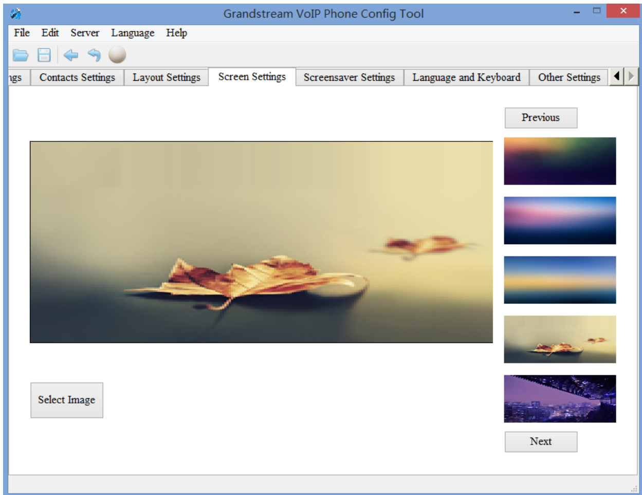
Figure 7: Screen Settings
