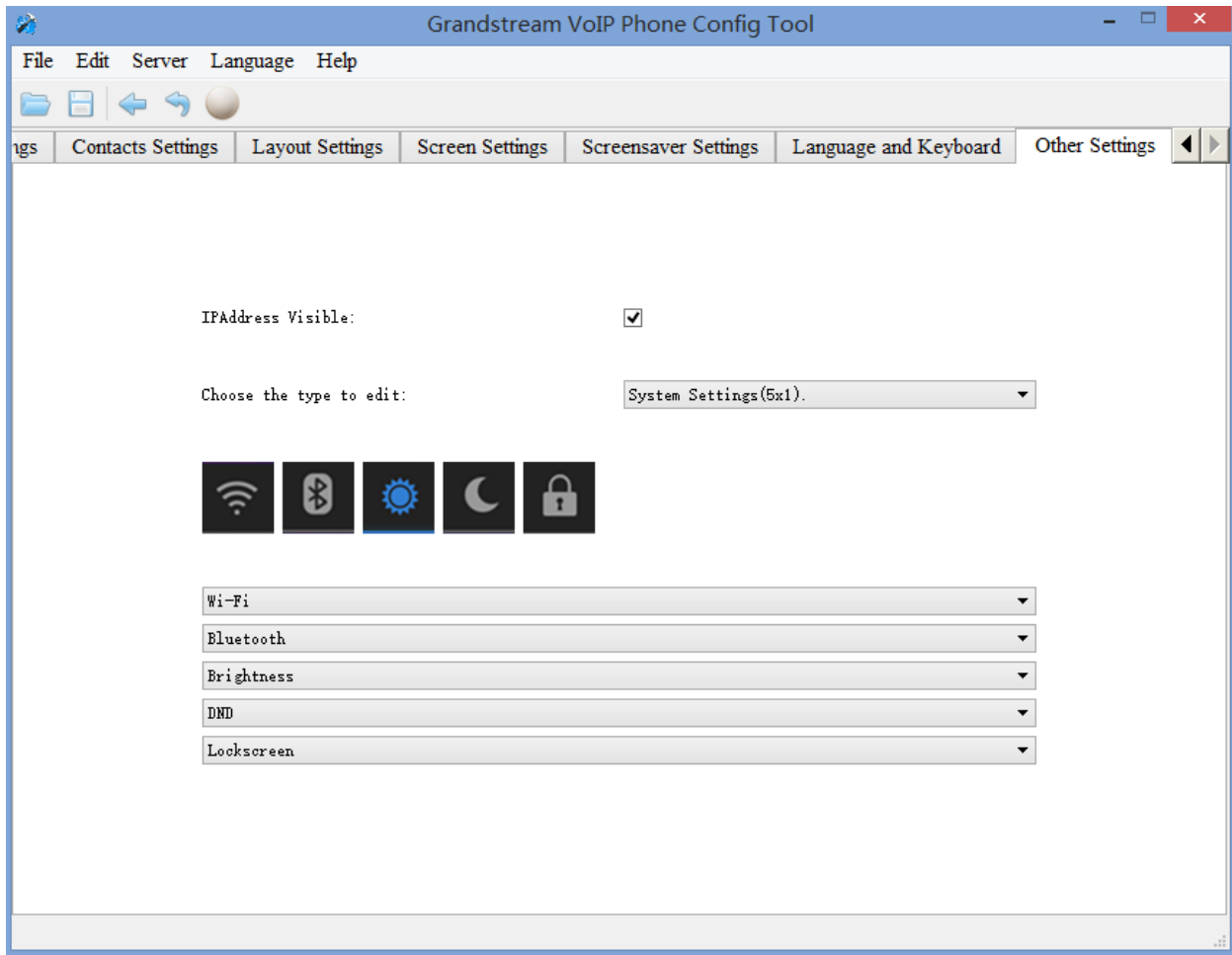
Figure 8: Other Settings
